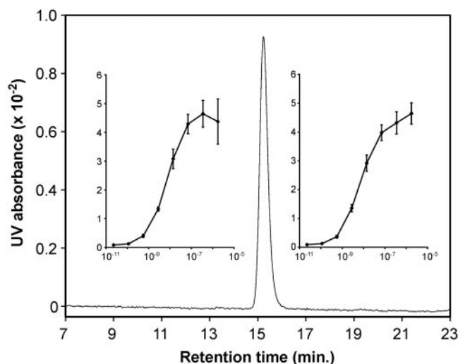
Fig. 5. Comparison of isolated vs. synthetic ITE. An HPLC chromatograph of a mixture of natural ( \approx 20 ng) and synthetic ( \approx 20 ng) ITE is shown. HPLC condition: C18 analytical column ( 4.6 \times 250 mm), methanol/water (70:30 vol/vol); flow rate = 0.5 ml/min; \lambda = 356 nm; x axis, retention time. y axis, UV absorbance. (Insets) Dose-response curves (mean \pm SD) generated by the natural (Left) and synthetic (Right) ITE, relative right units (ordinate) vs. agonist concentration.
